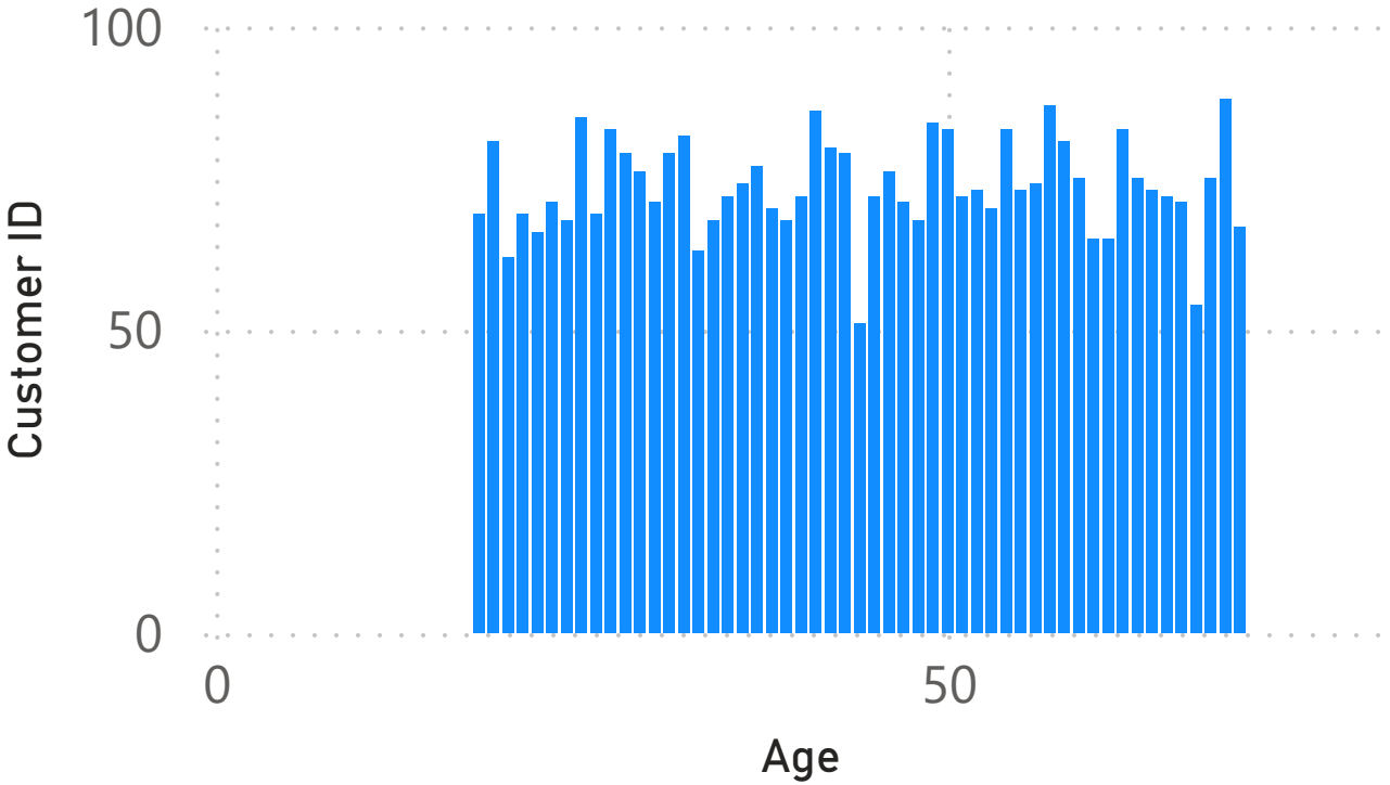
Customer Age Distribution
